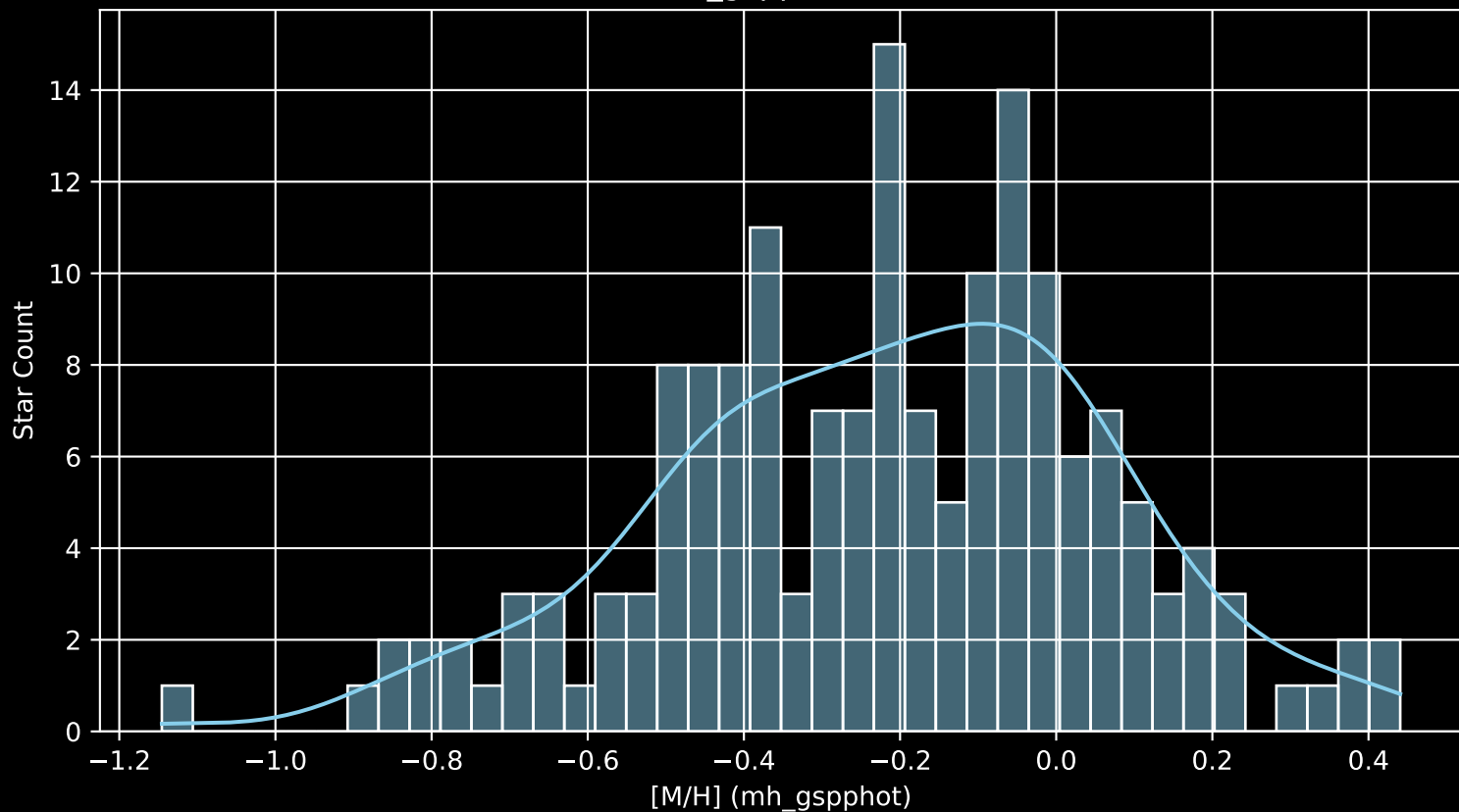
APOGEE DR17 Field: [271-32-O_TESS [M/H] (mh_gspphot) (n= 169)
