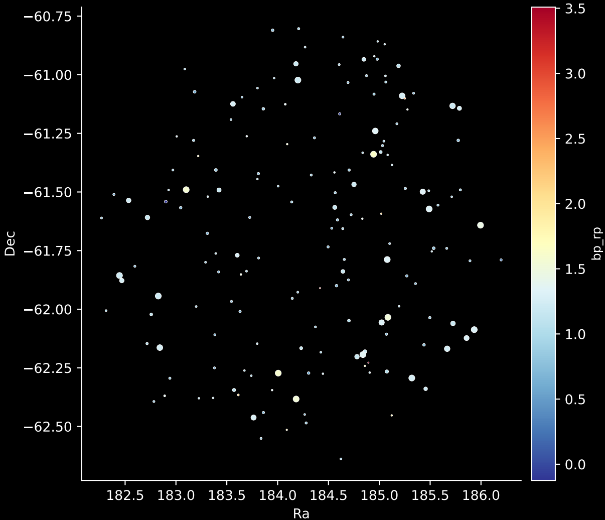
APOGEE DR17 Field: [271-32-O_TESS] Stars: 171
