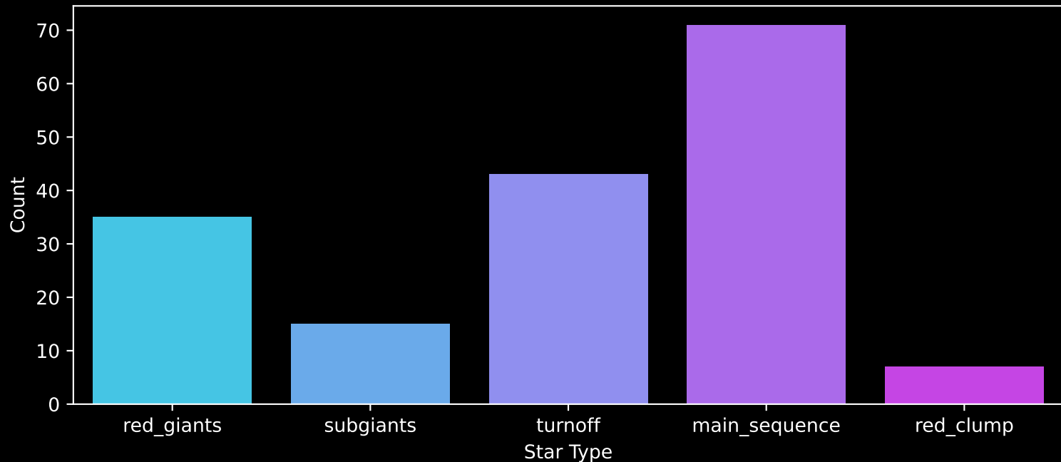
APOGEE DR17 Field: [271-32-O_TESS] Count plot of Star Type
