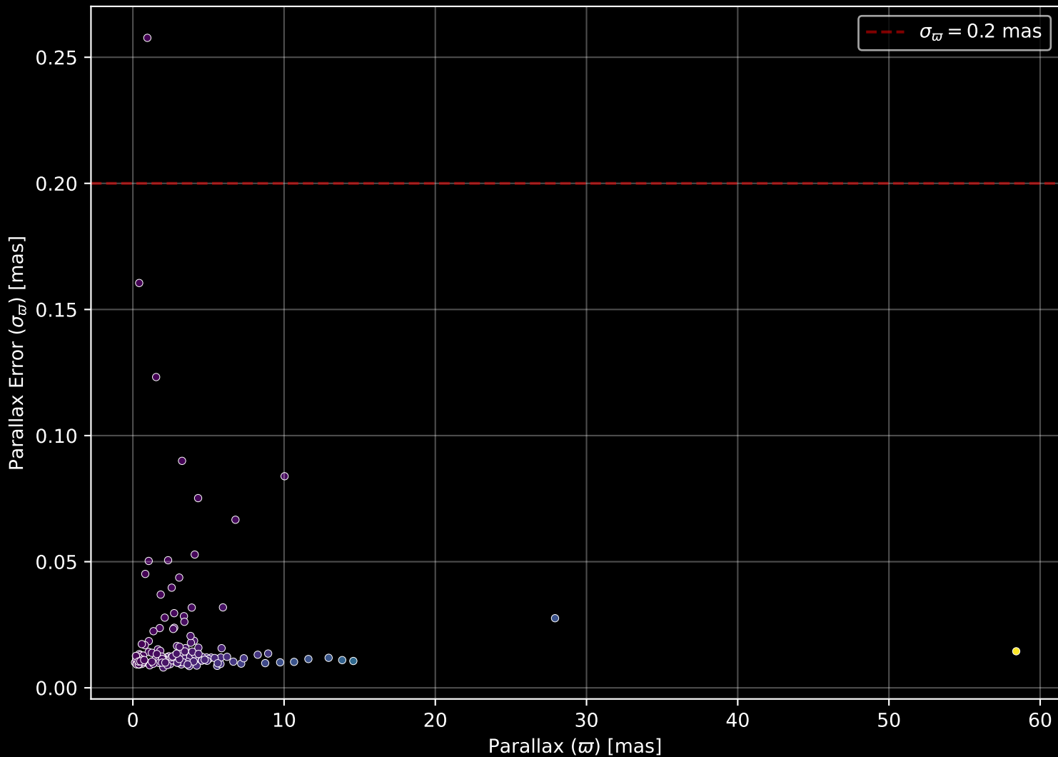
APOGEE DR17 Field: [271-32-O_TESS] Parallax Quality (n= 171)
