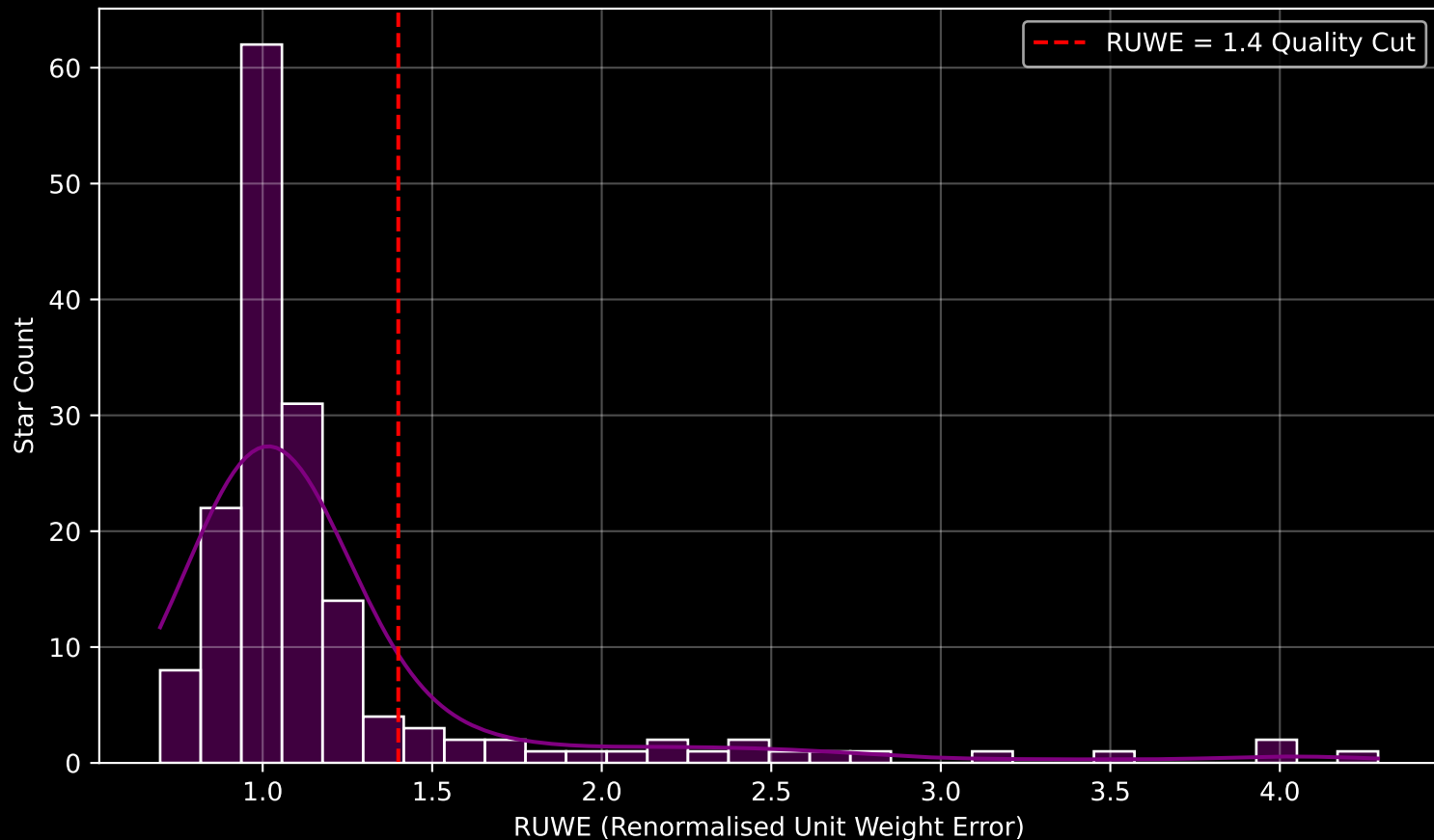
GAPOGEE DR17 Field [271-32-O_TESS] RUWE Distribution (n= 164)
