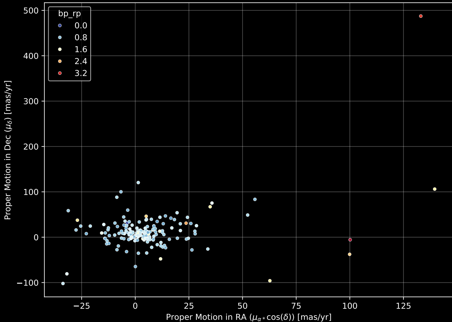
APOGEE DR17 Field: [271-32-O_TESS] Proper Motion Diagram (n= 171)
